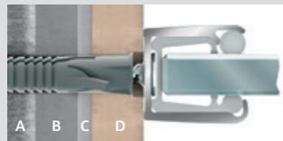
A) Wall B) Plaster C) Tile adhesive D) Wall tile
