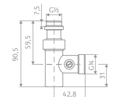
Special return valve
